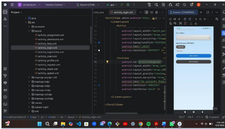
Figure 12.ASSIGNMENT BUTTON
