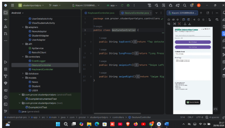
Figure 29 swipe gesture
