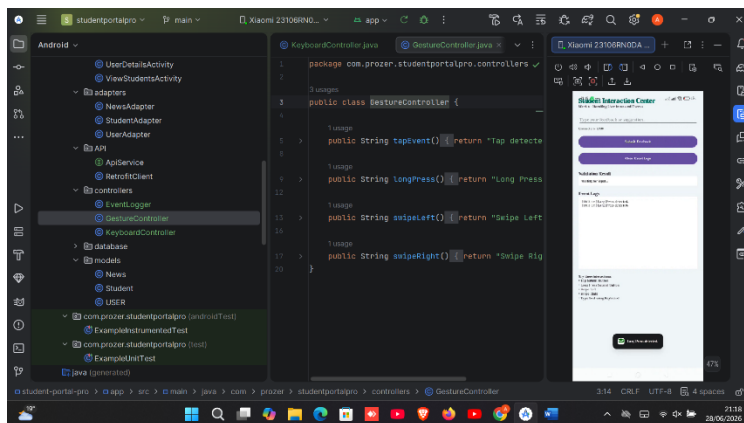
Figure 31 longpress gesture
