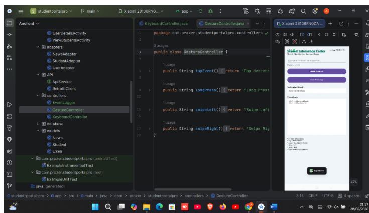
Figure 30 tap gesture
